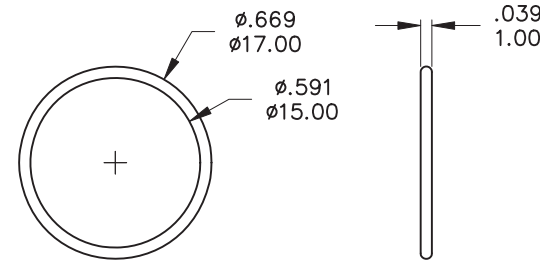
O-RINGx1/pcs FCP-P004
