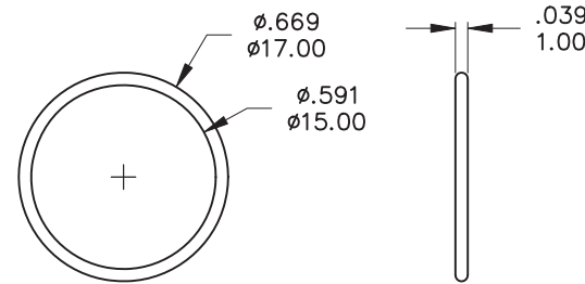
O-RINGx1 FCP-P004
