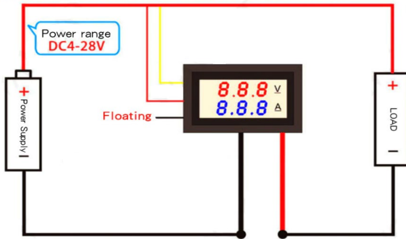
1. Directly powered wiring diagrams for gauge 1A or 10A headers
