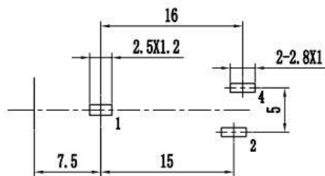
P. C. B LAYOUT (TOP VIEW) Tolerance: ±0.05
