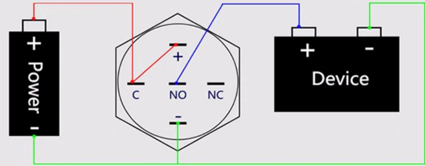
Wiring diagram 2:
