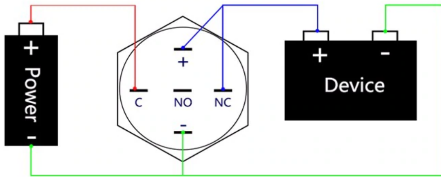
Wiring diagram 3:
