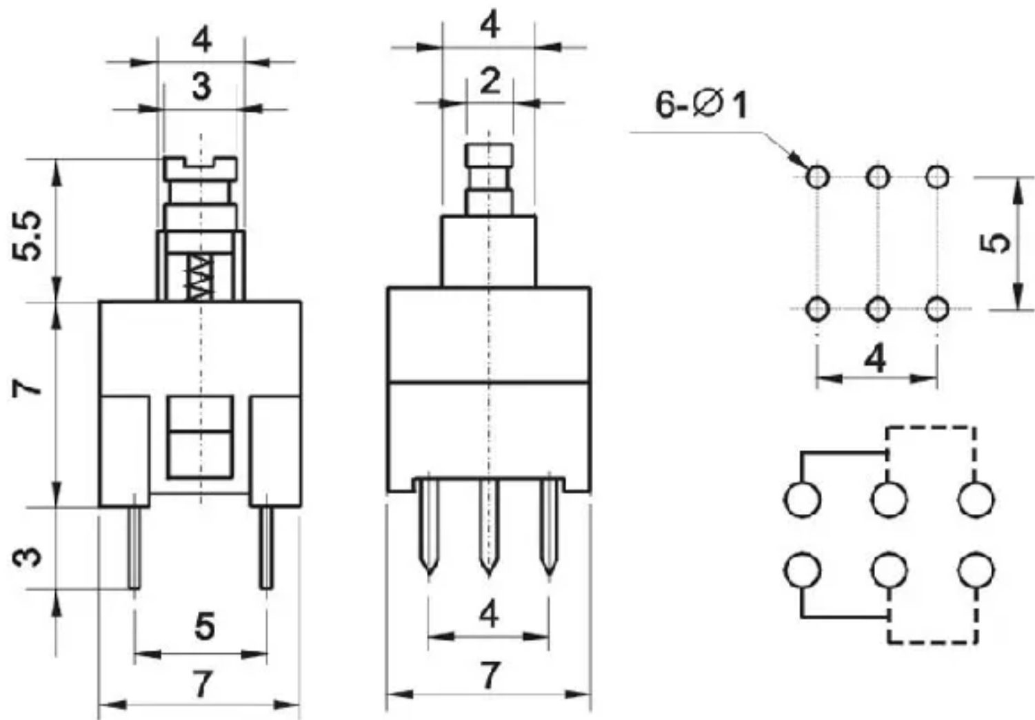
Dimension in mm±0.5mm
