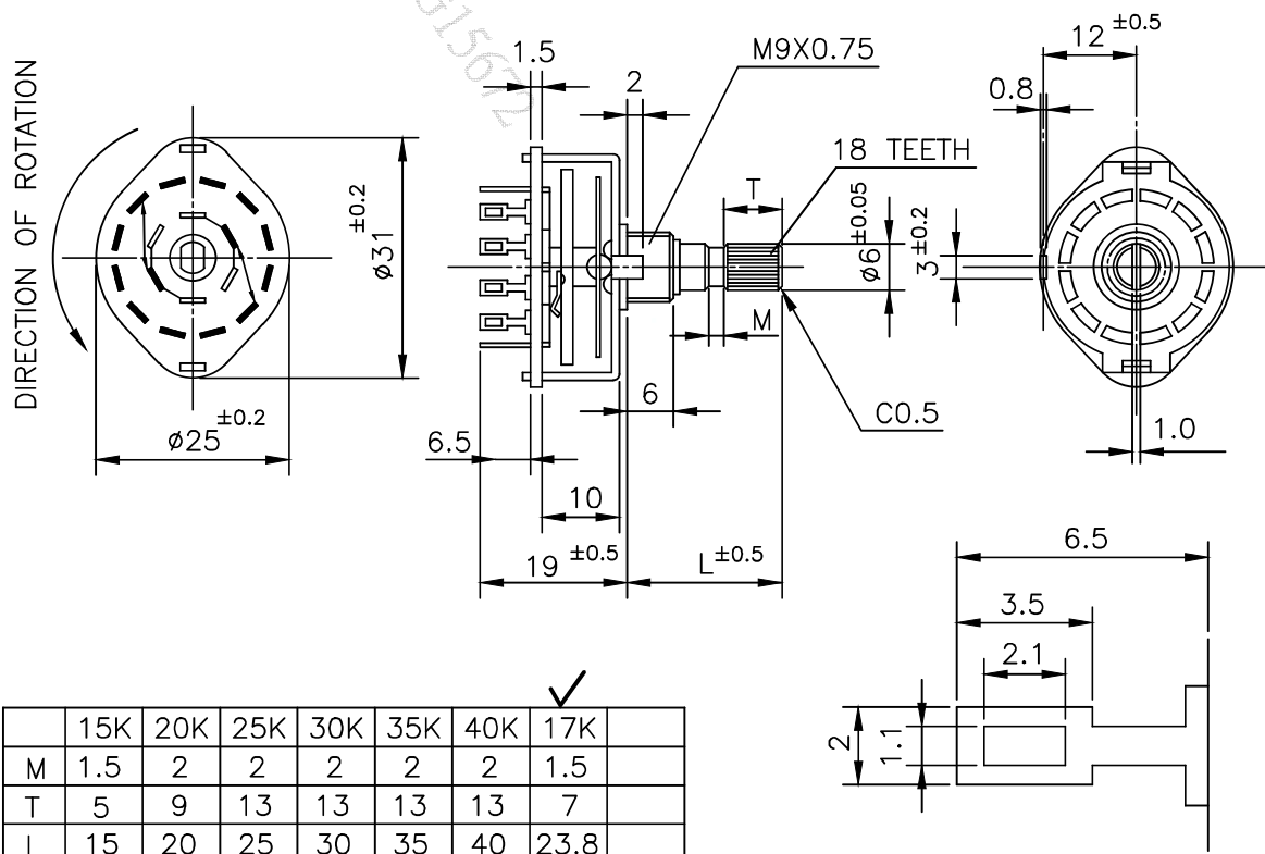
DETAIL OF TERMINAL(5/1)
