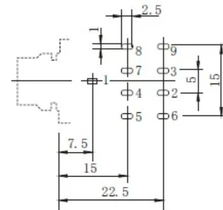
P. C. B LAND PATTERN
