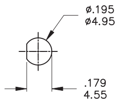
PANEL MOUNTING
