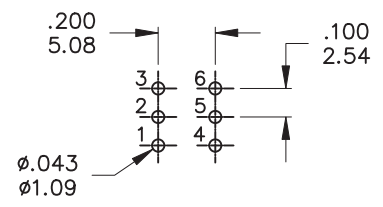
P.C. MOUNTING
