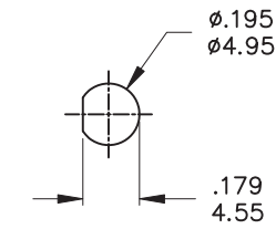
PANEL MOUNTING
