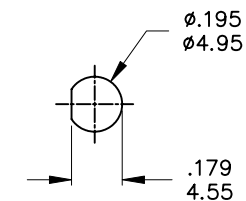
PANEL MOUNTING
