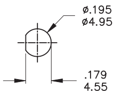
PANEL MOUNTING
