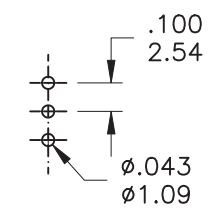
P.C. MOUNTING
