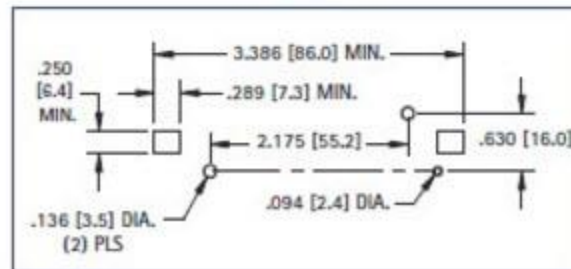
Pad Layout
