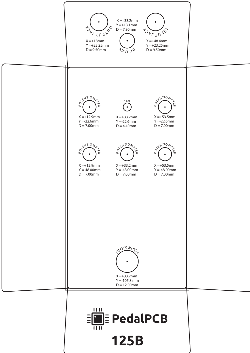
PedalPCB 5-Knob Type 1
