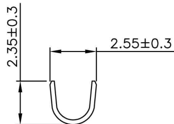
B-B SEC
