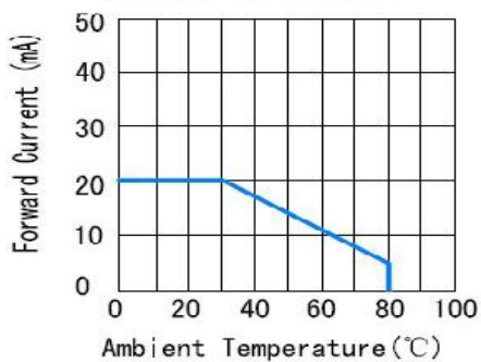
ALLOWABLE FORWARD CURRENT AMBIENT TEMPERATURE
