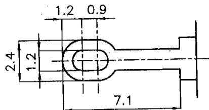
DETAIL OF TERMINAL(5/1)
