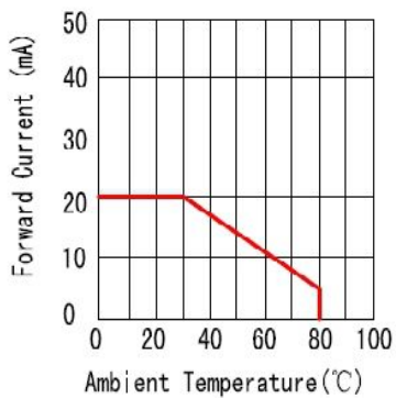
ALLOWABLE FORWARD CURRENT vs. AMBIENT TEMPERATURE
