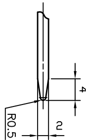
TERMTNAL DETAIL
