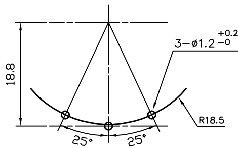
P.C.B MOUNTING HOLE DETAIL VIEWED FROM MOUNTING SIDE
