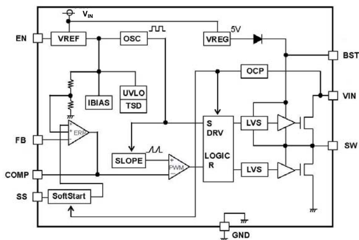
Figure 3. Block Diagram
