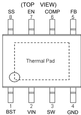
Figure 2. Pin Configuration
