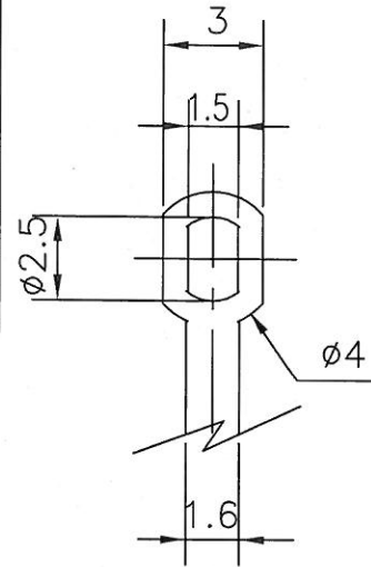
TERMINAL DETAIL (4/1)
