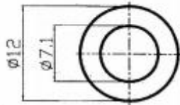
WASHER 1 PC t=0.4
